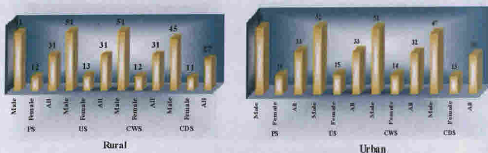
Chart 6.2.3 : WPR in different approaches
