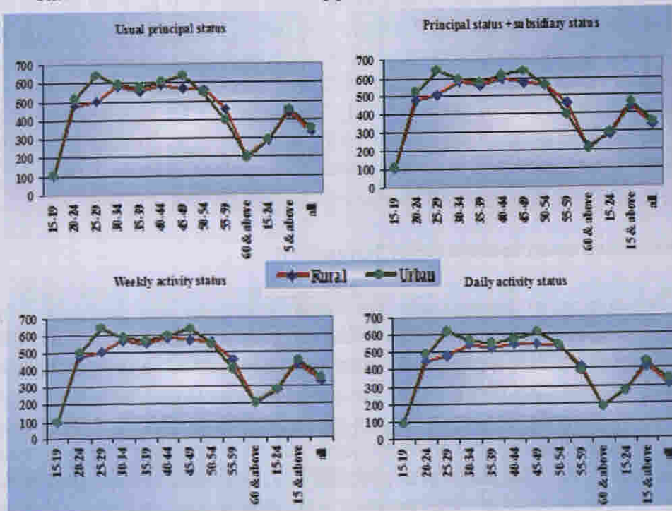
Chart 6.2.2: LFPR in different approaches for different age groups
