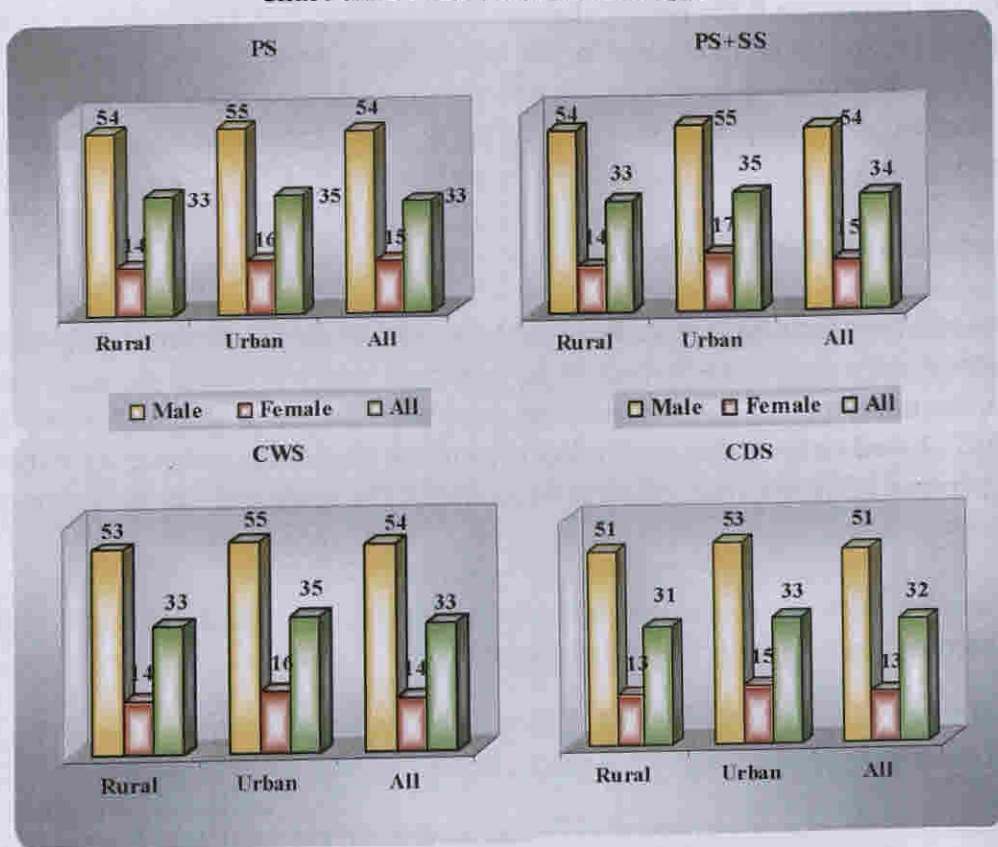
Chart 6.2.1 : LFPR in different approaches
